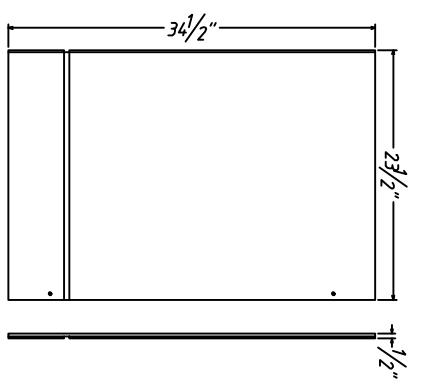
BACK PANEL
