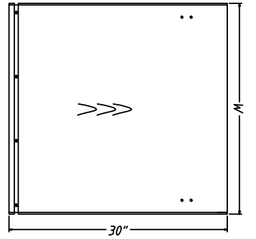
BACK PANEL
