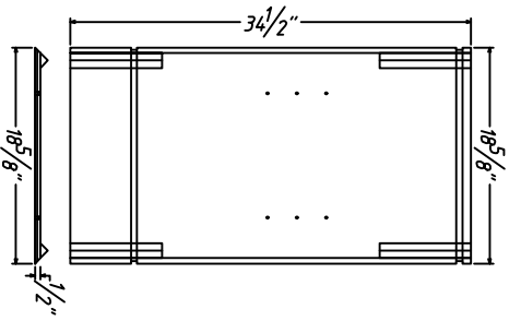
BACK PANEL
